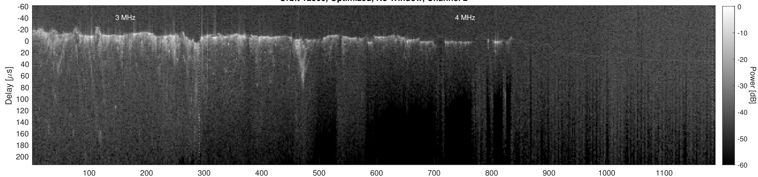
Orbit 12566, Cluttergram
