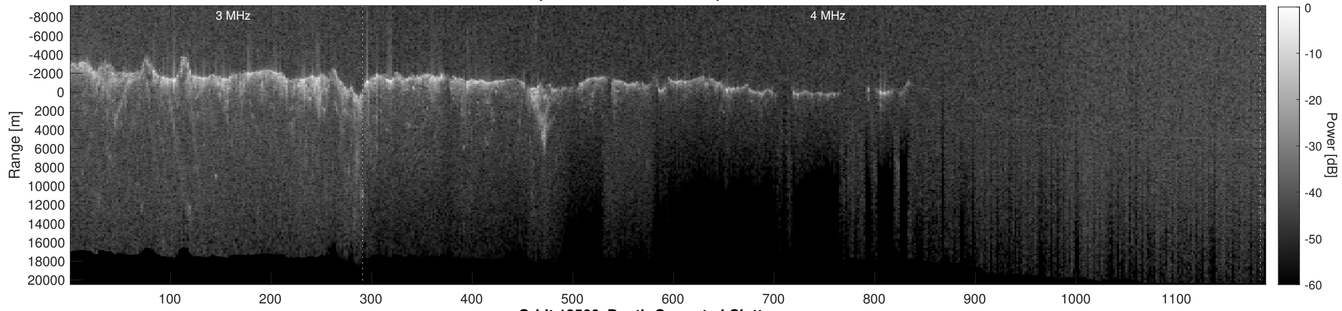
Orbit 12566, Depth-Corrected Cluttergram
