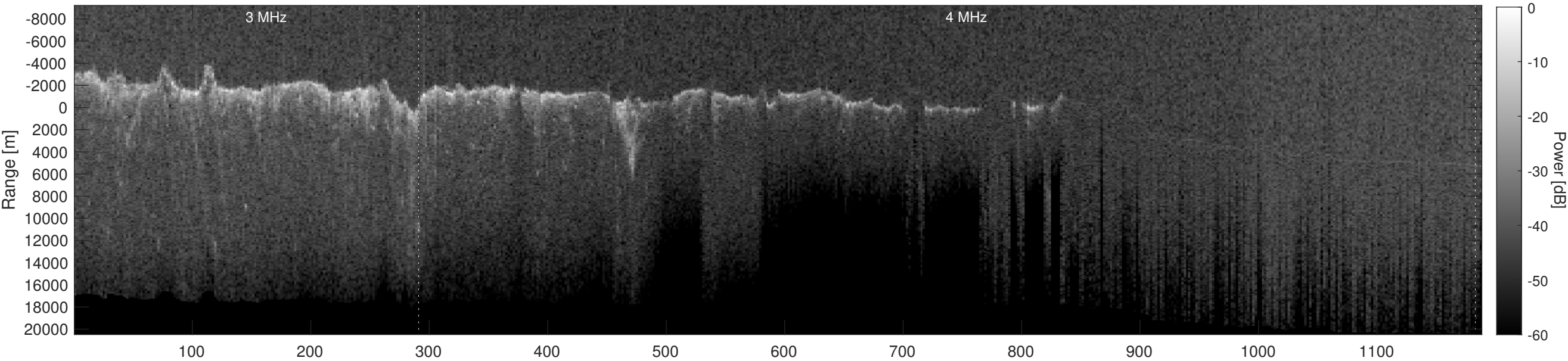
Orbit 12566, Depth-Corrected Cluttergram
