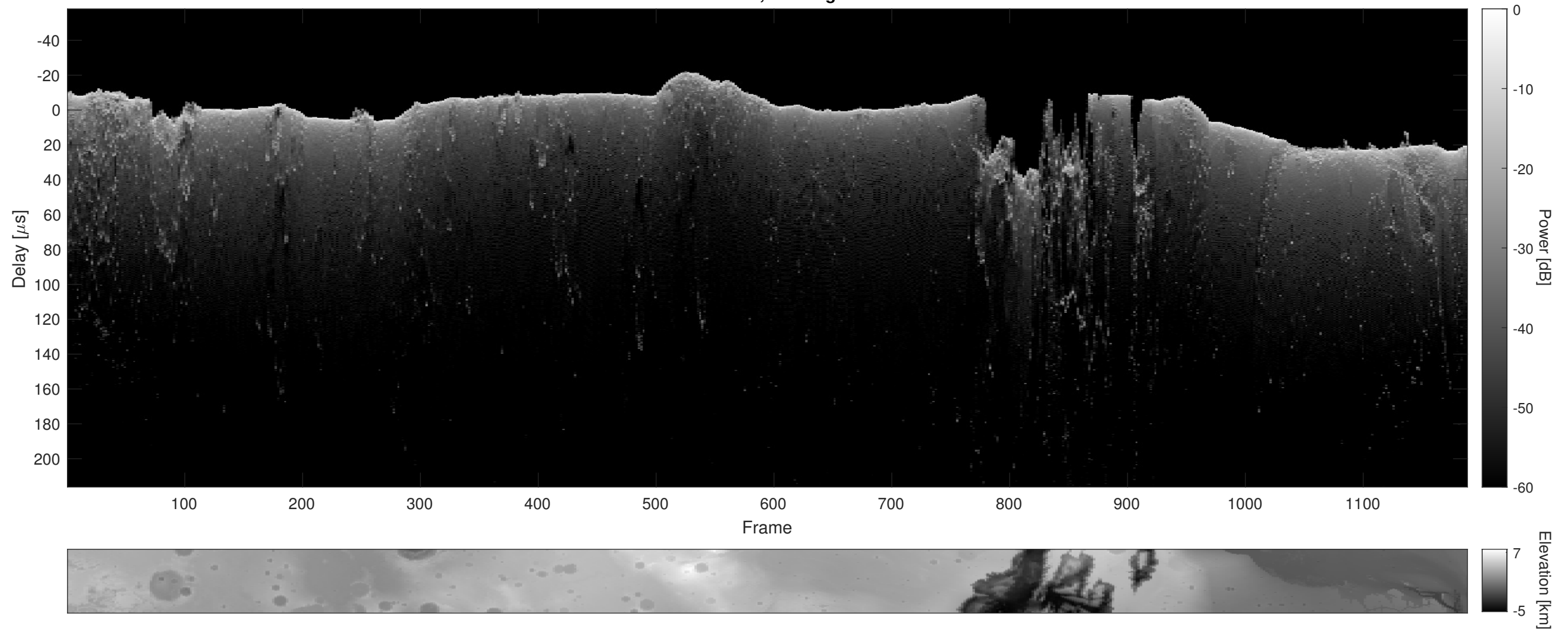
Orbit 12568, Cluttergram
