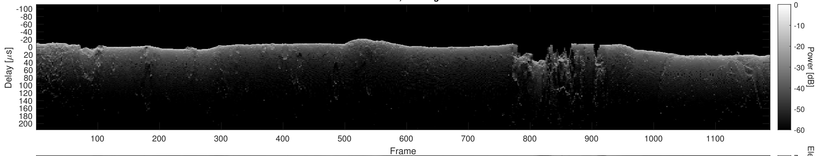
Orbit 12568, Cluttergram
