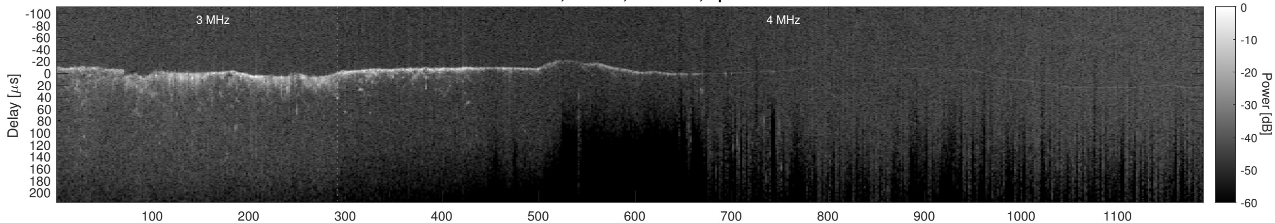
Orbit 12568, Cluttergram
