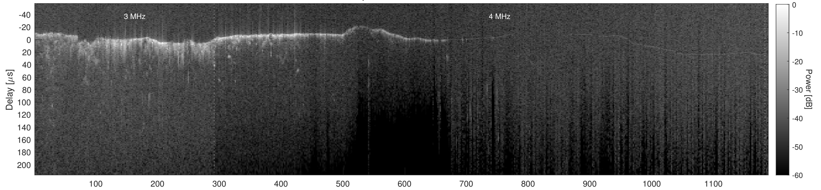
Orbit 12568, Cluttergram
