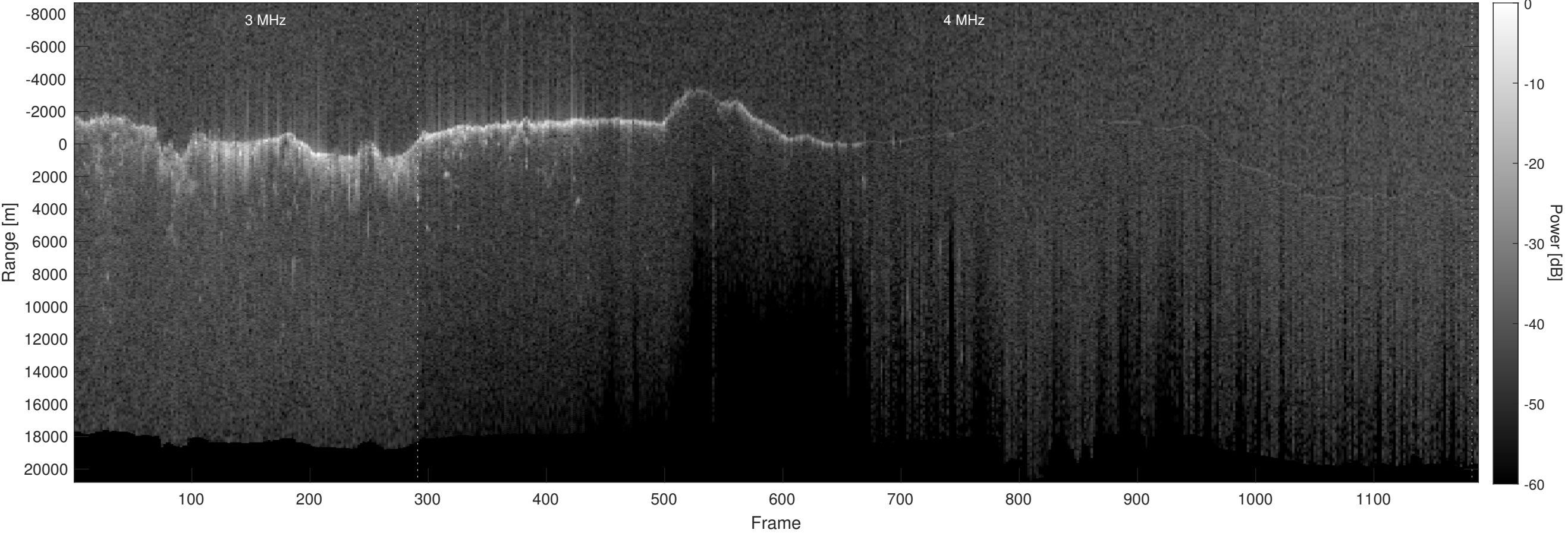
Orbit 12568, Optimized, No Window, Depth-Corrected, Channel 2
