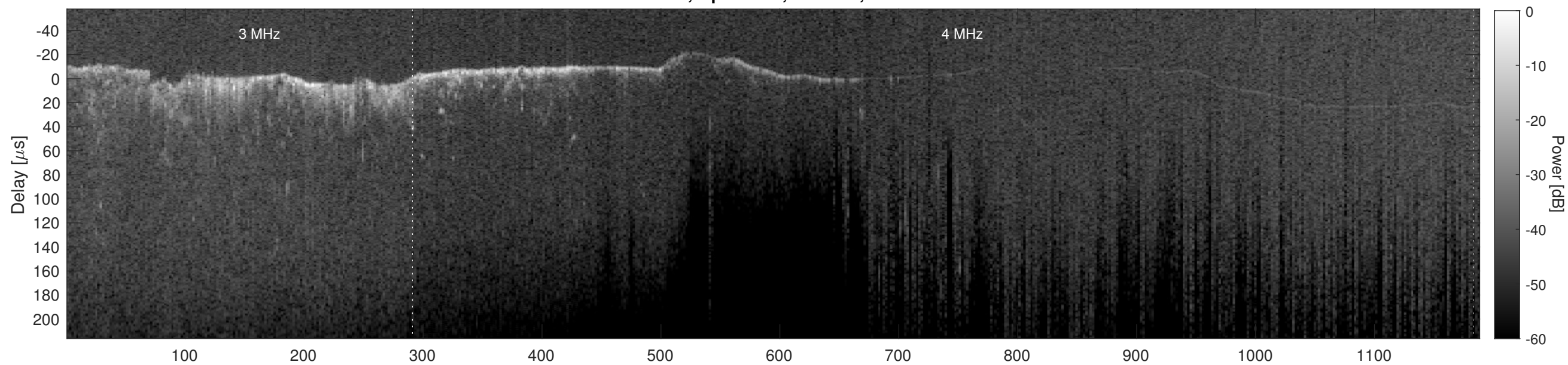
Orbit 12568, Cluttergram
