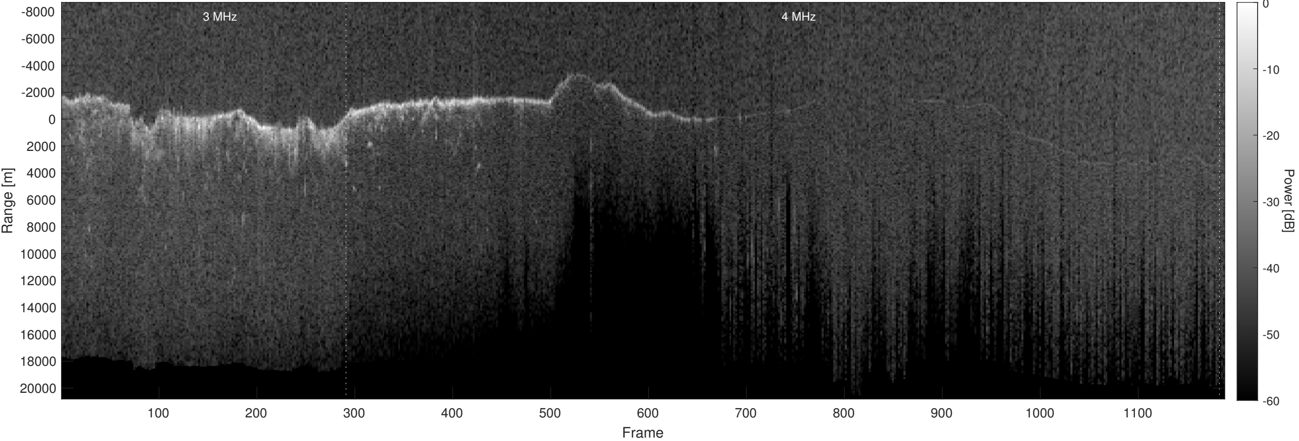
Orbit 12568, Optimized, Window, Depth-Corrected, Channel 2
