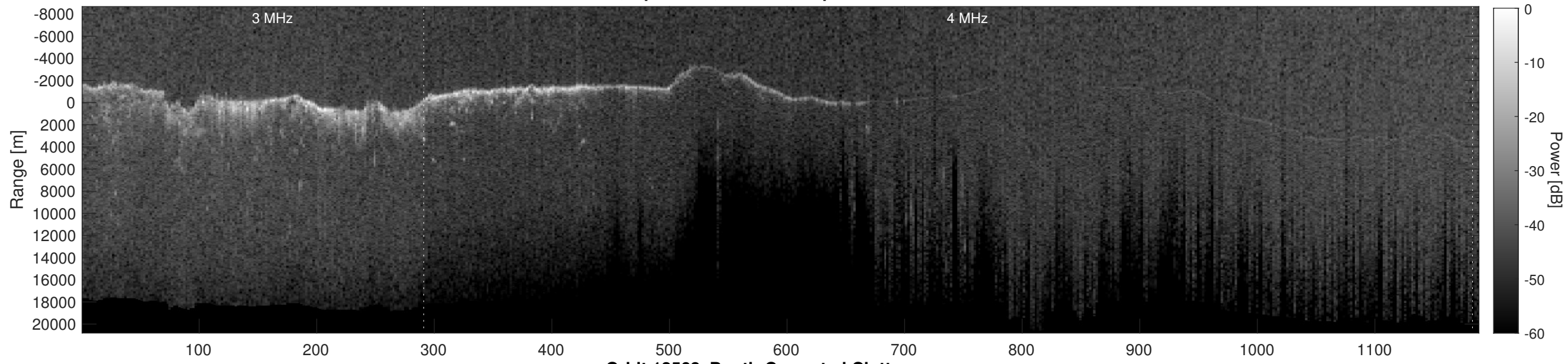
Orbit 12568, Depth-Corrected Cluttergram
