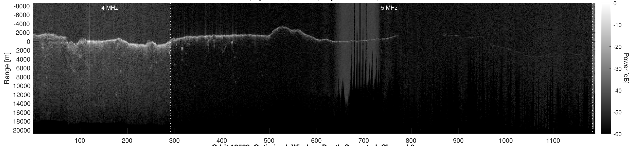
Orbit 12568, Optimized, Window, Depth-Corrected, Channel 2
