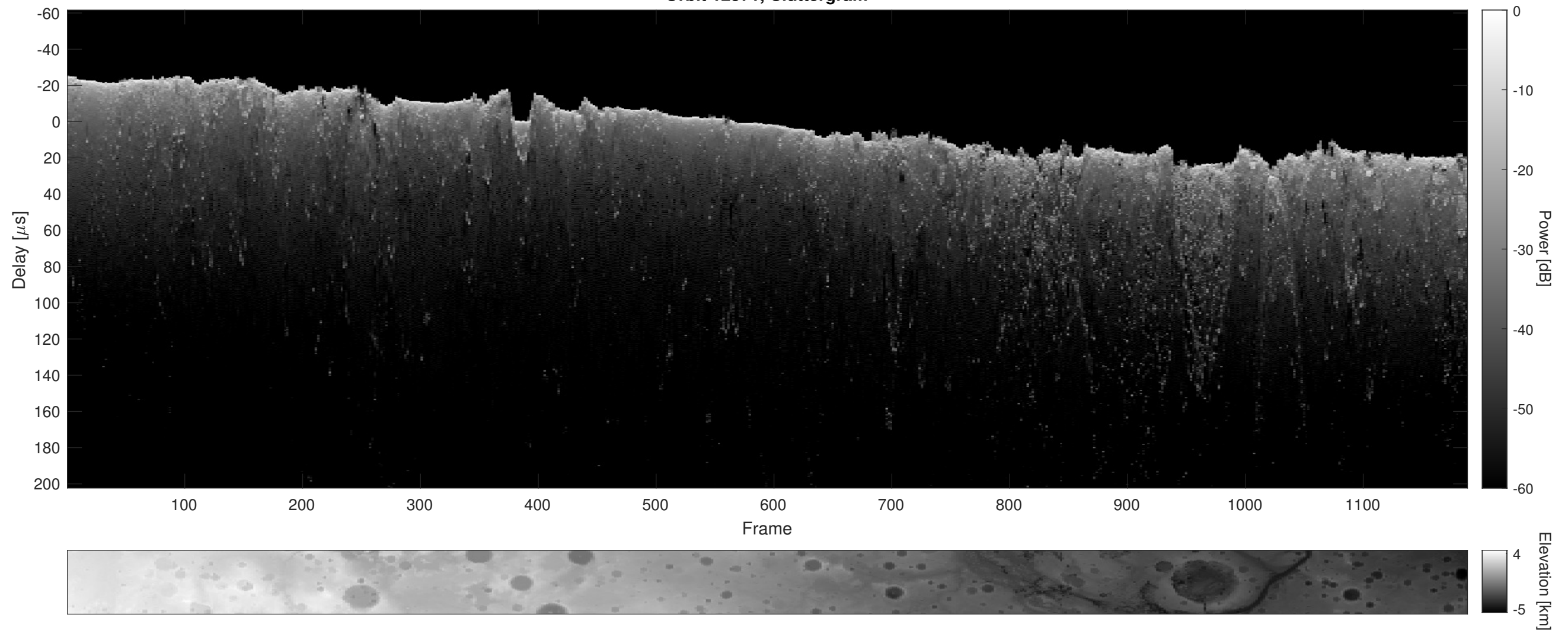
Orbit 12571, Cluttergram
