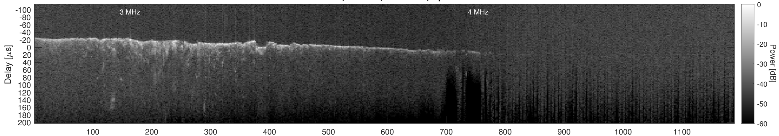
Orbit 12571, Cluttergram
