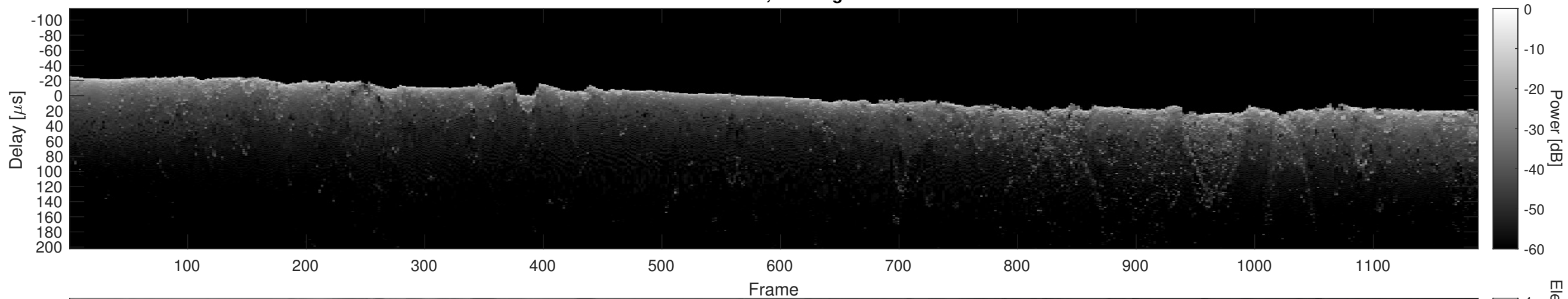
Orbit 12571, Cluttergram
