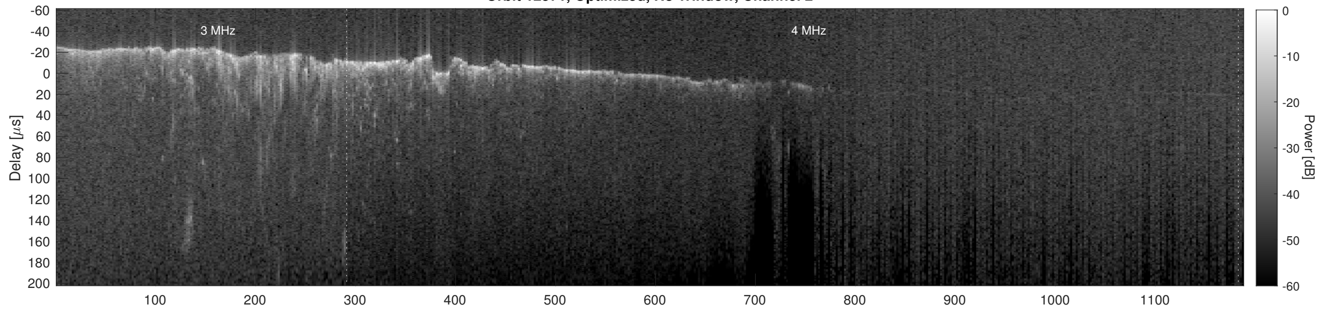
Orbit 12571, Cluttergram
