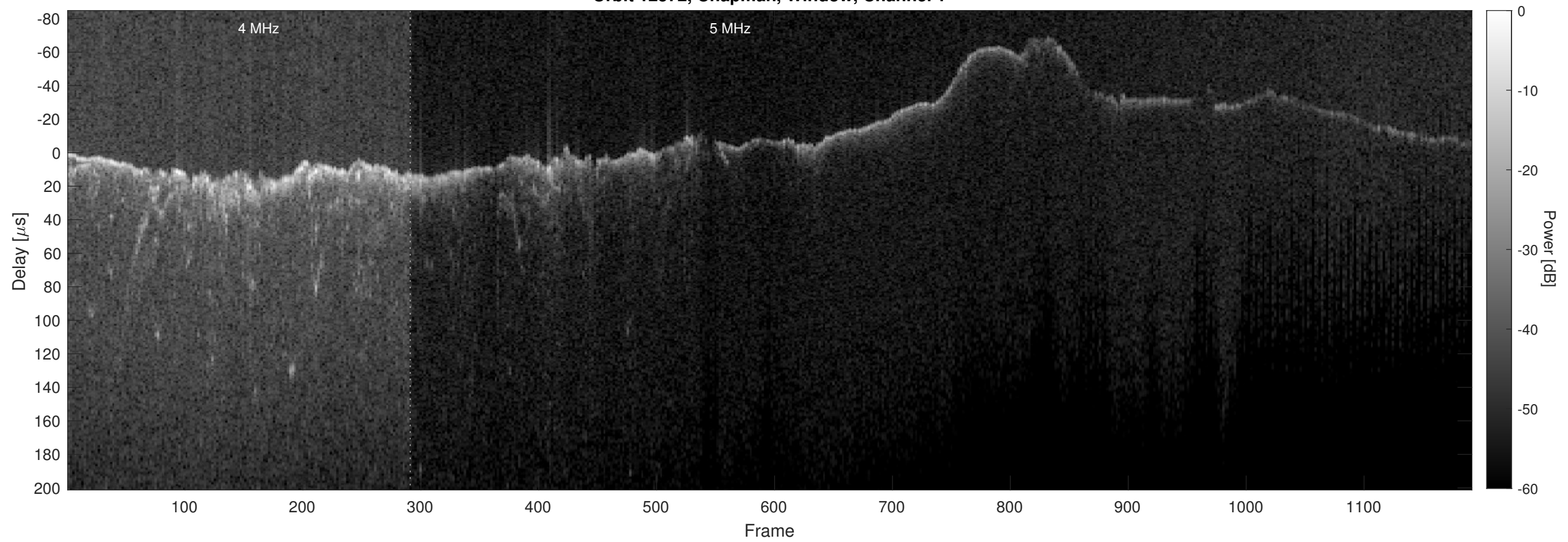
Orbit 12572, Chapman, Window, Channel 2
