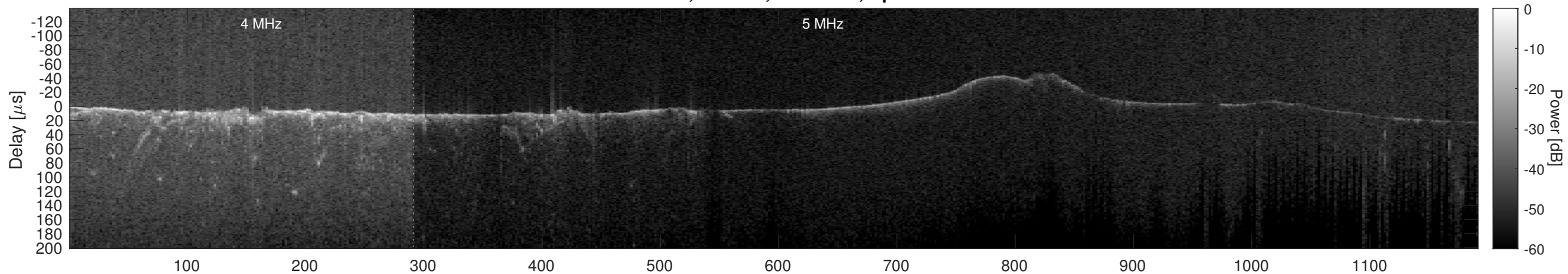
Orbit 12572, Cluttergram
