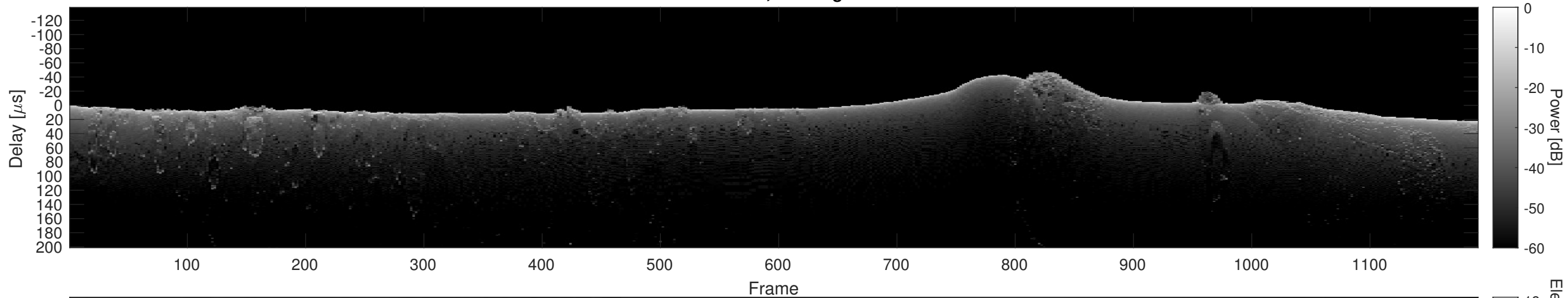
Orbit 12572, Cluttergram
