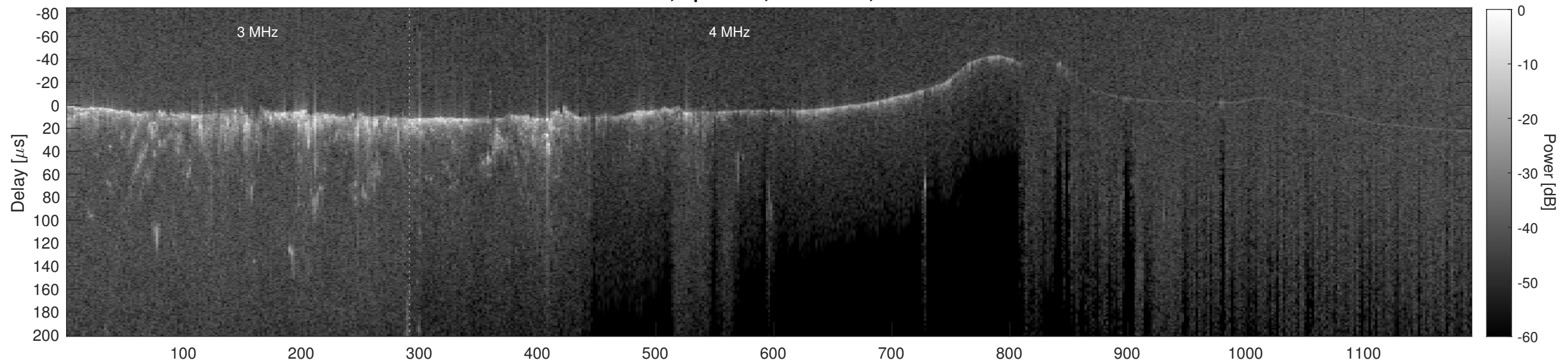
Orbit 12572, Cluttergram
