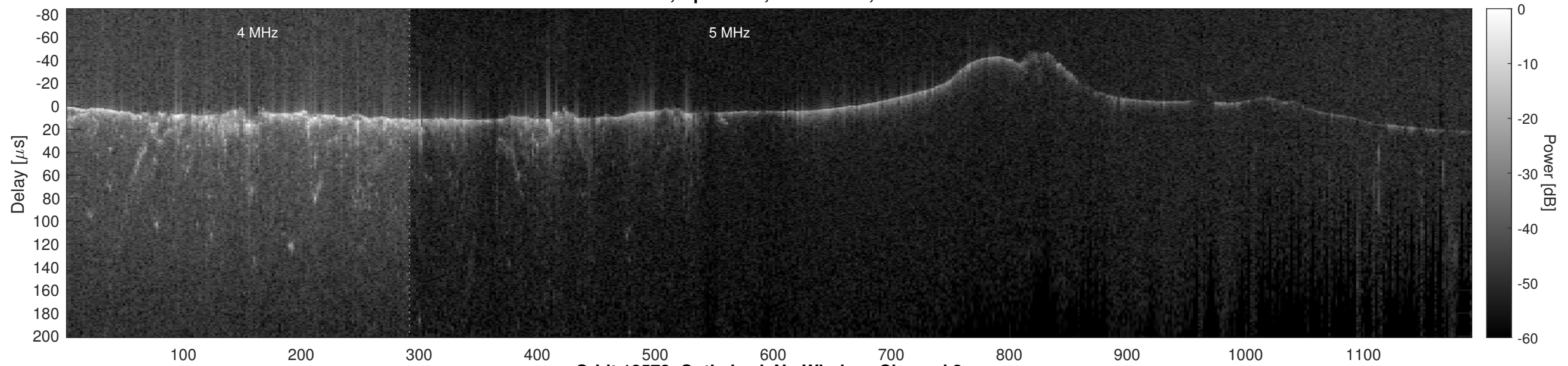
Orbit 12572, Optimized, No Window, Channel 2
