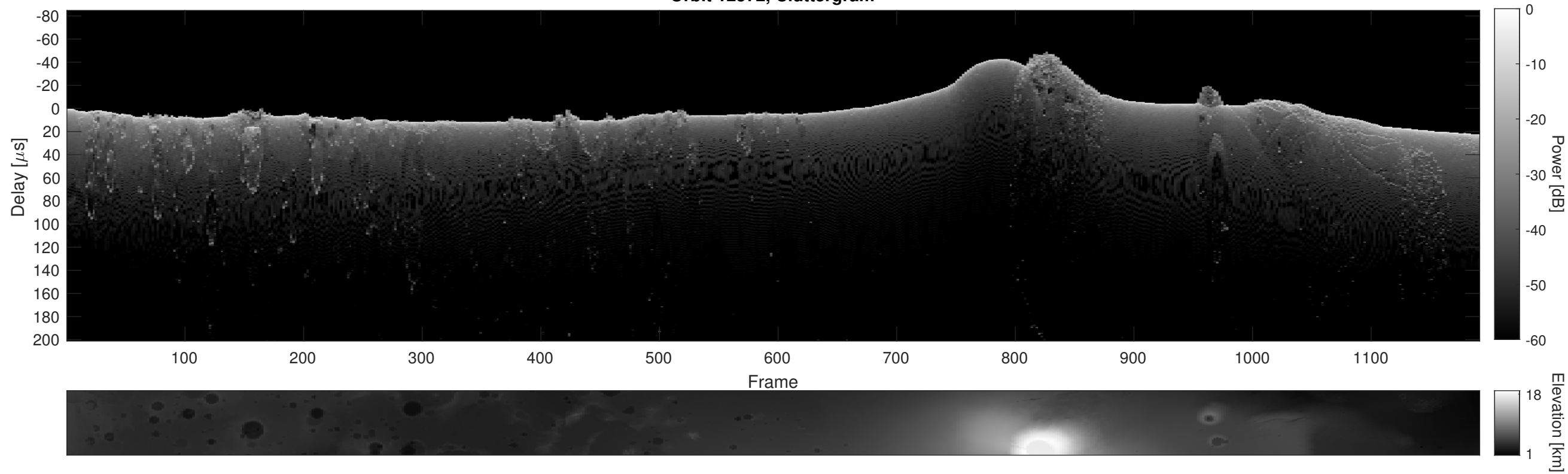
Orbit 12572, Cluttergram
