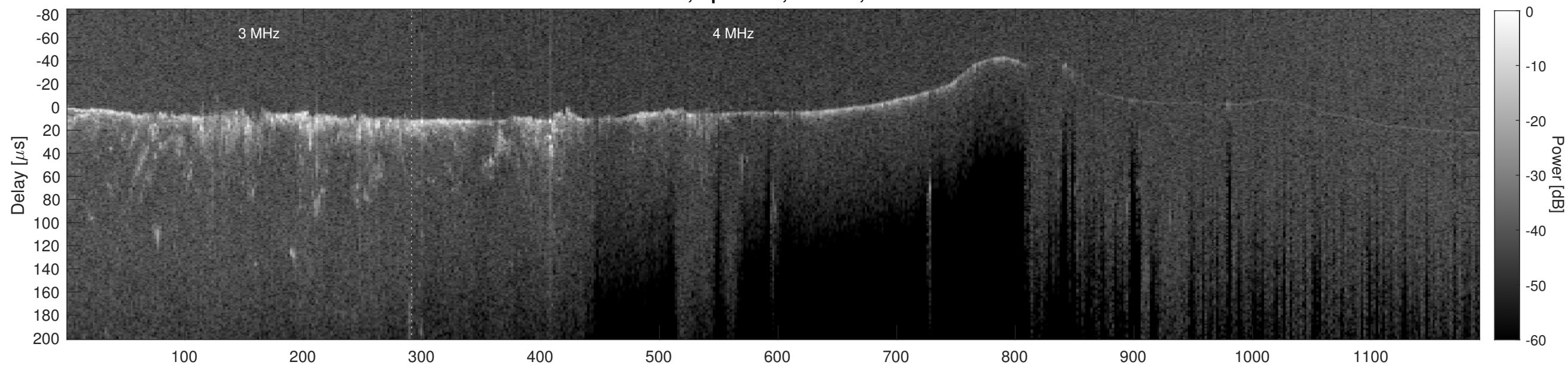
Orbit 12572, Cluttergram
