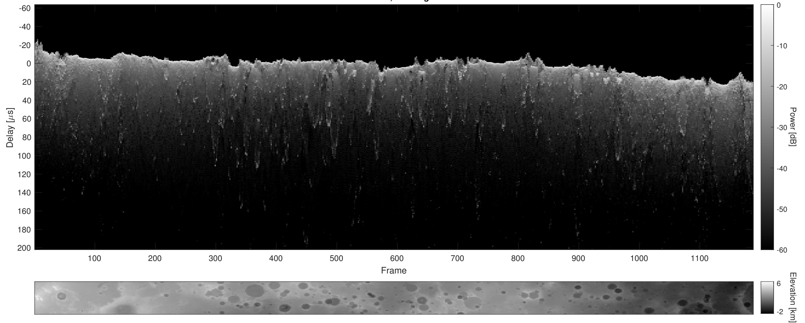
Orbit 12574, Cluttergram
