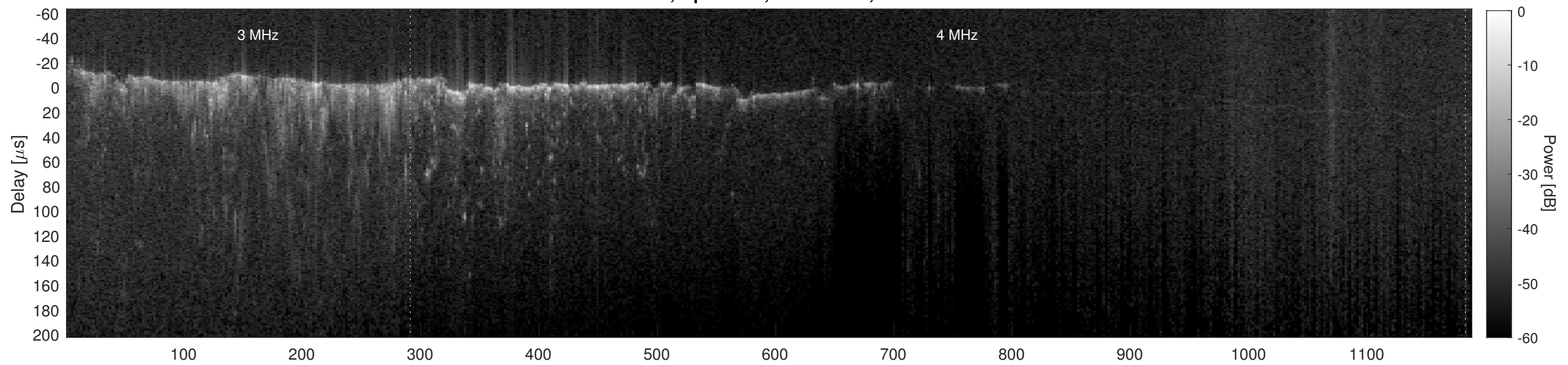
Orbit 12574, Cluttergram
