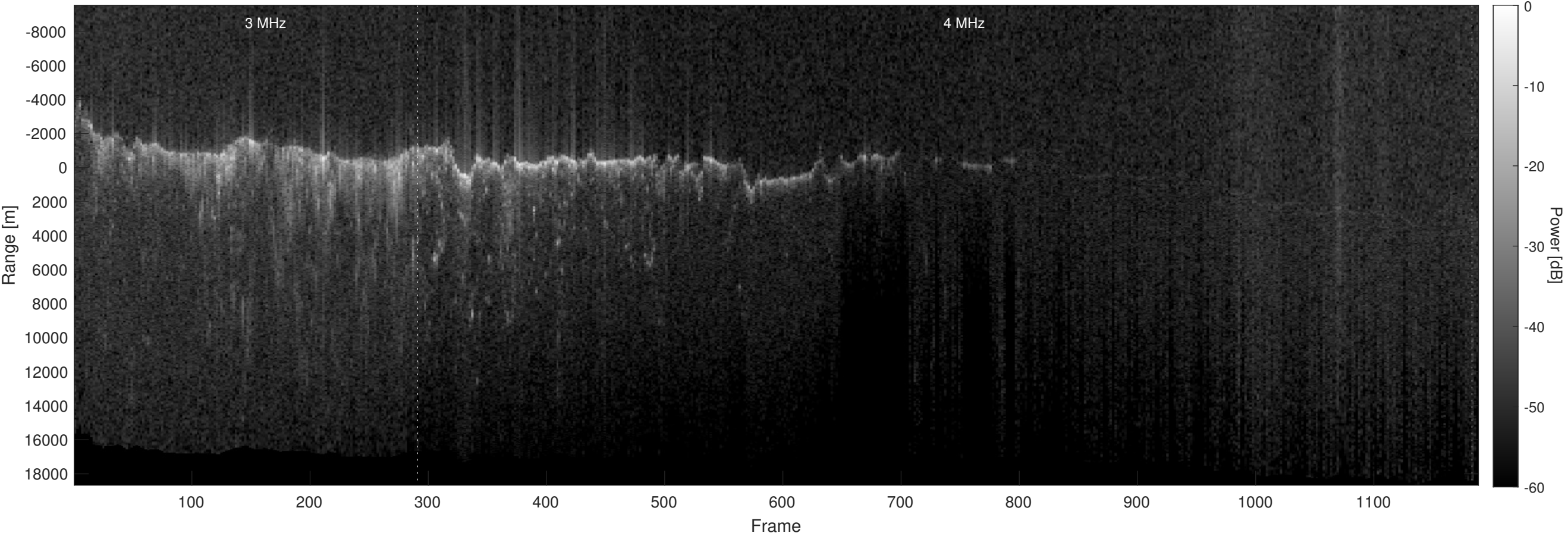
Orbit 12574, Optimized, No Window, Depth-Corrected, Channel 2
