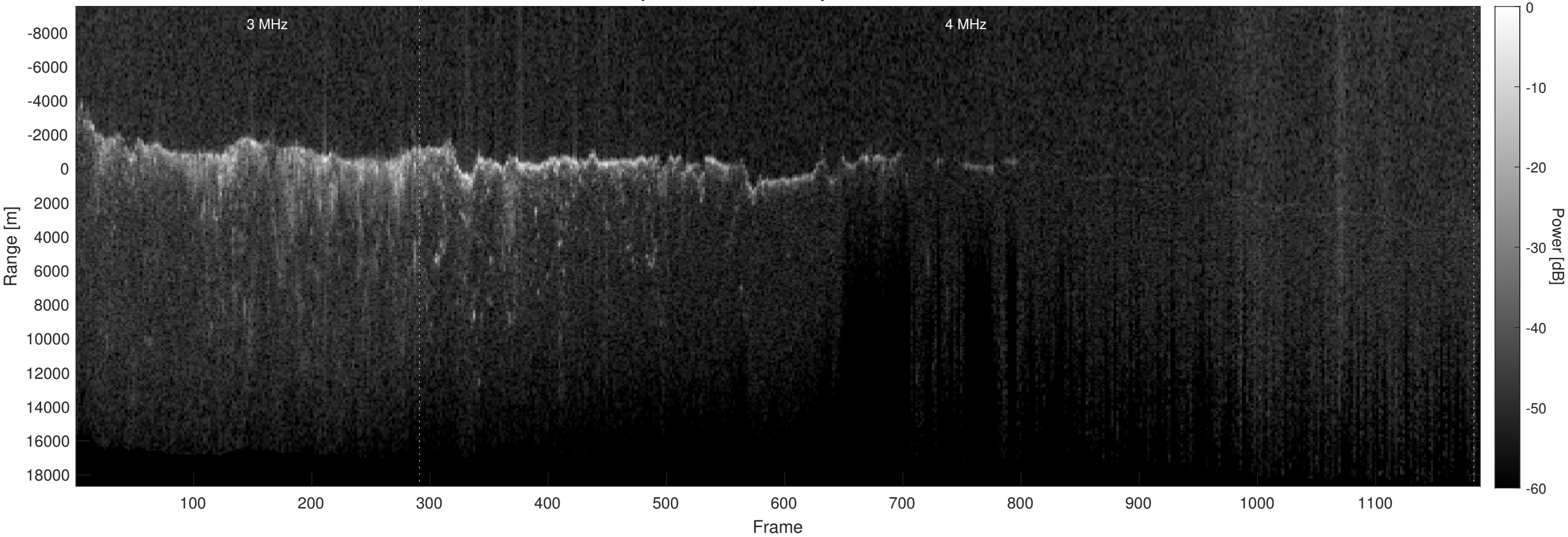
Orbit 12574, Optimized, Window, Depth-Corrected, Channel 2
