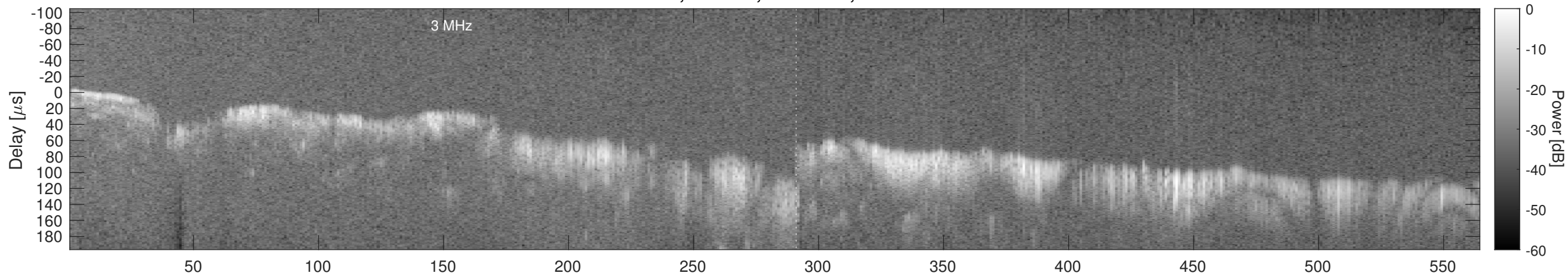
Orbit 12576, Window, Channel 2, Chapman
