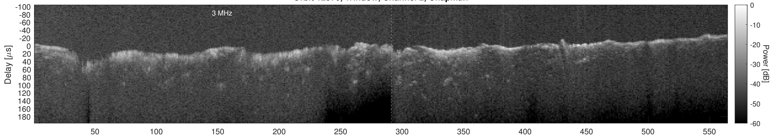
Orbit 12576, Window, Channel 2, Optimized
