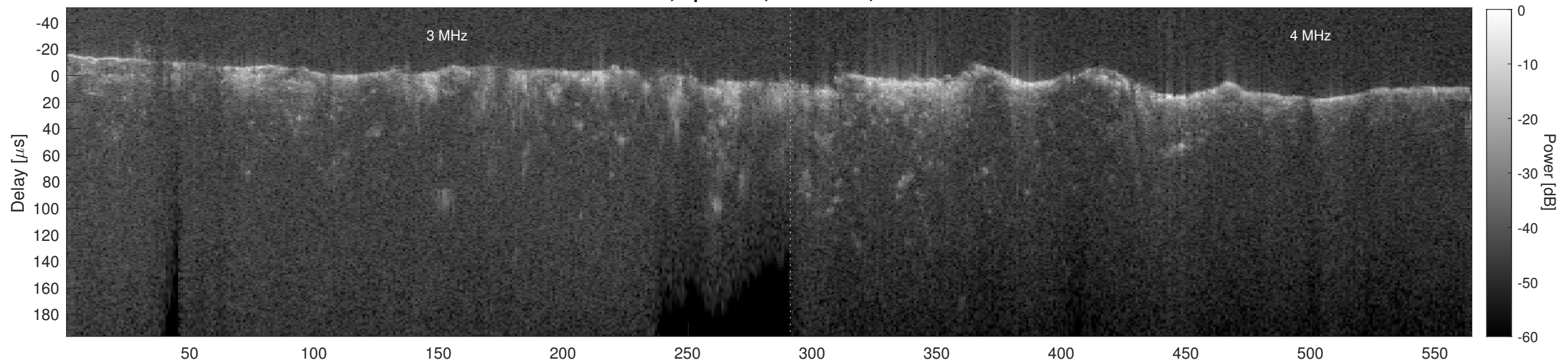
Orbit 12576, Cluttergram
