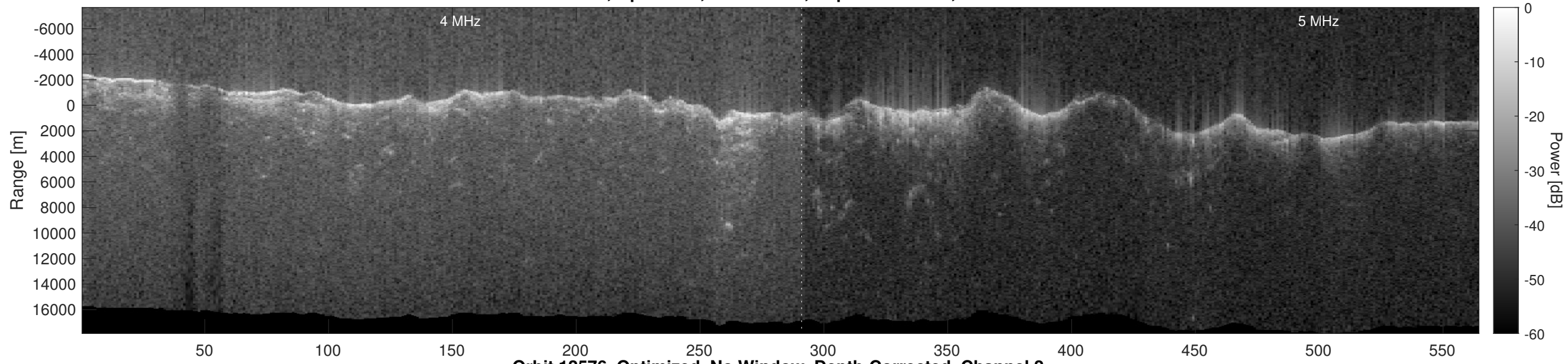
Orbit 12576, Optimized, No Window, Depth-Corrected, Channel 2
