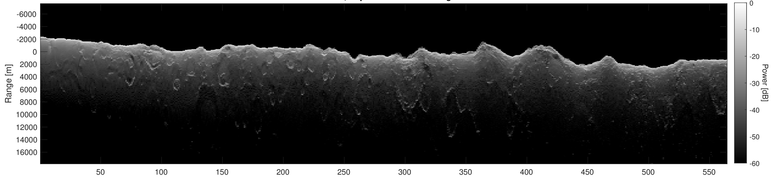
Orbit 12576, Depth-Corrected Cluttergram
