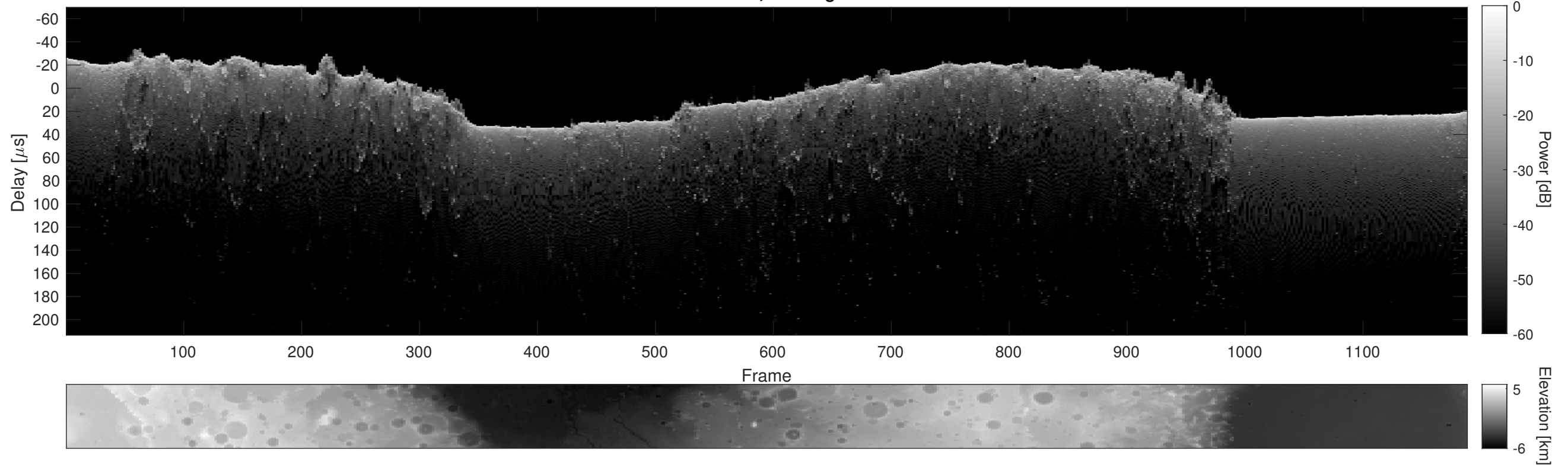
Orbit 12577, Cluttergram
