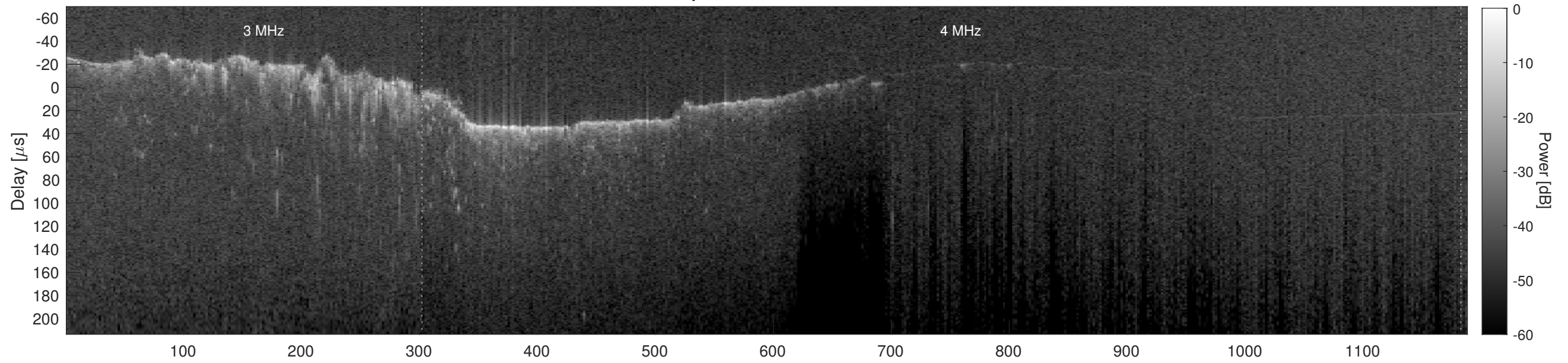
Orbit 12577, Cluttergram
