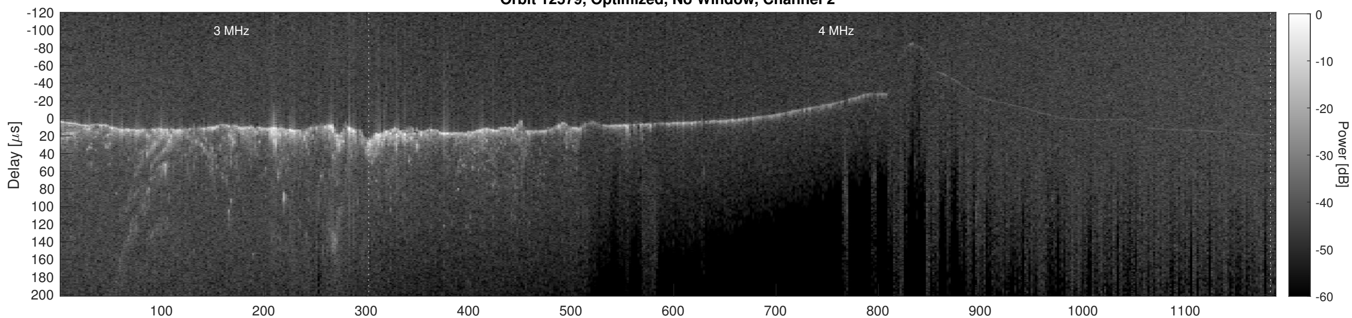
Orbit 12579, Cluttergram
