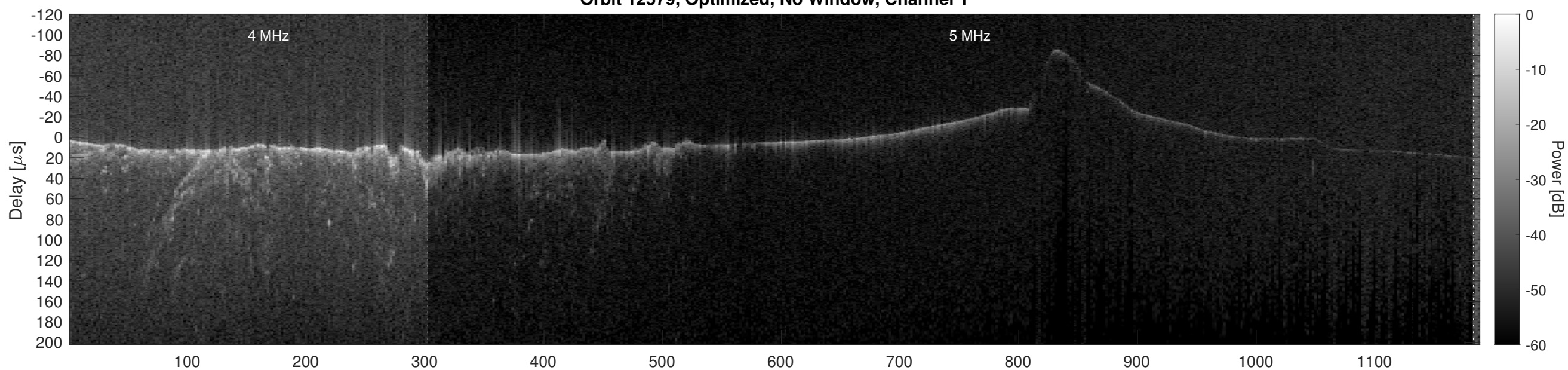
Orbit 12579, Optimized, No Window, Channel 2
