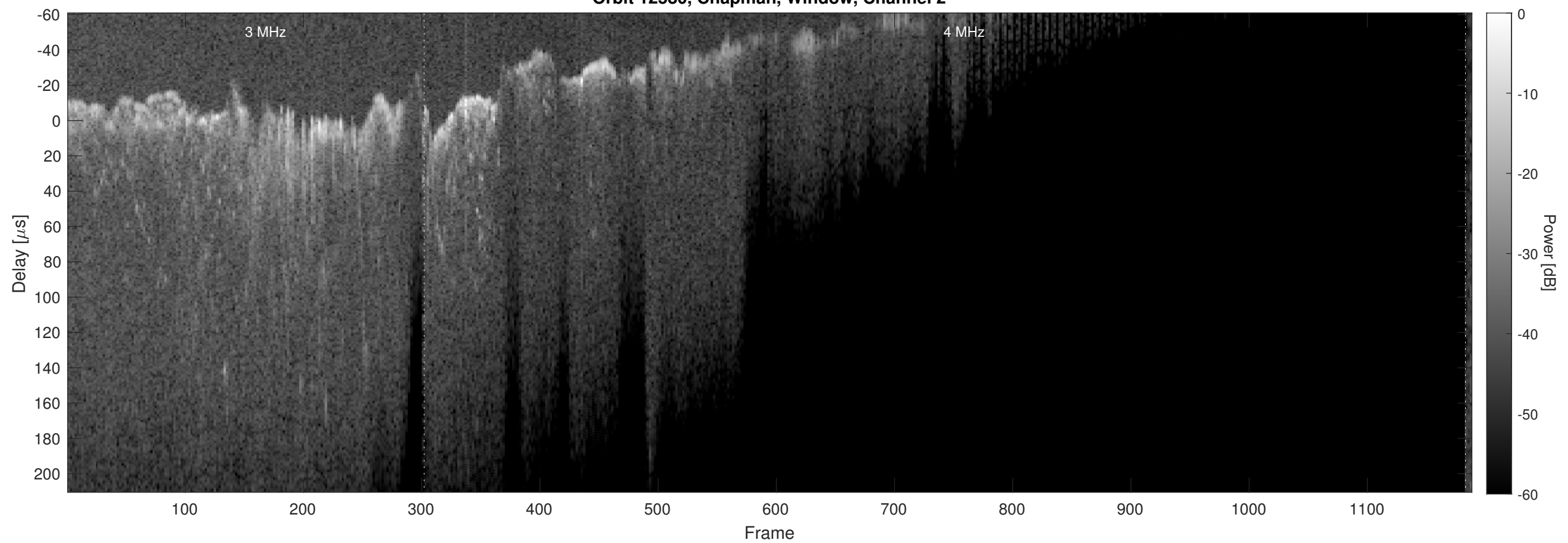
Orbit 12580, Chapman, Window, Channel 2
