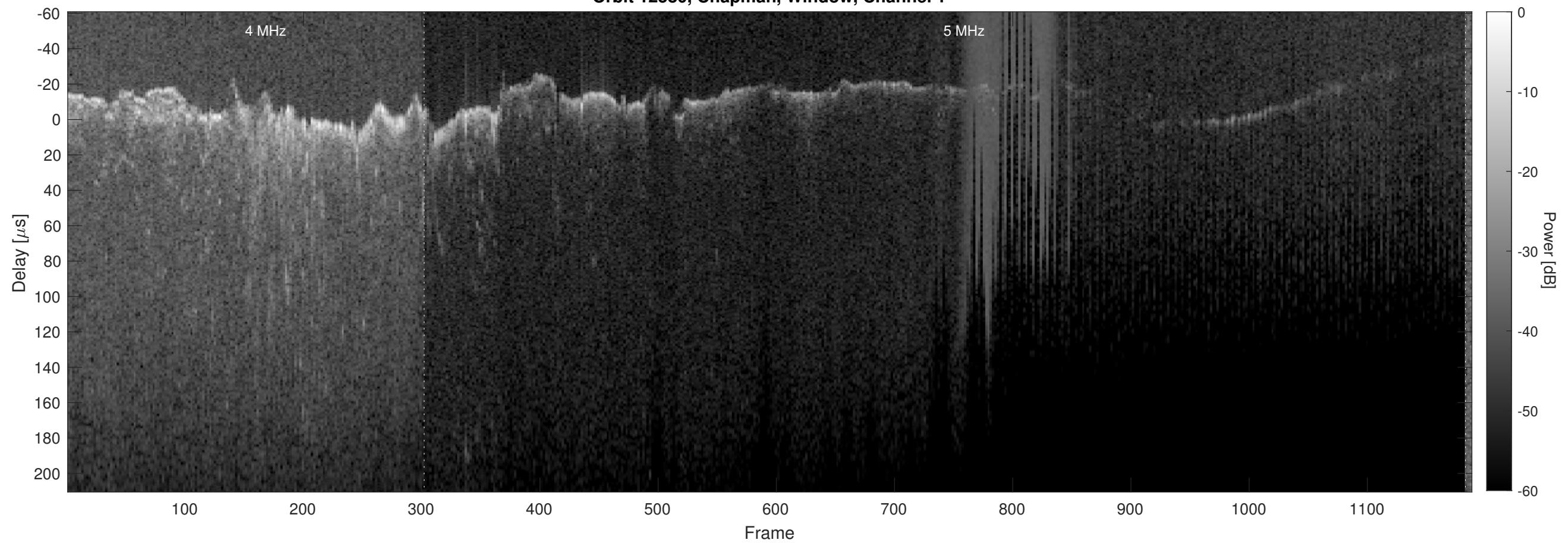
Orbit 12580, Chapman, Window, Channel 2
