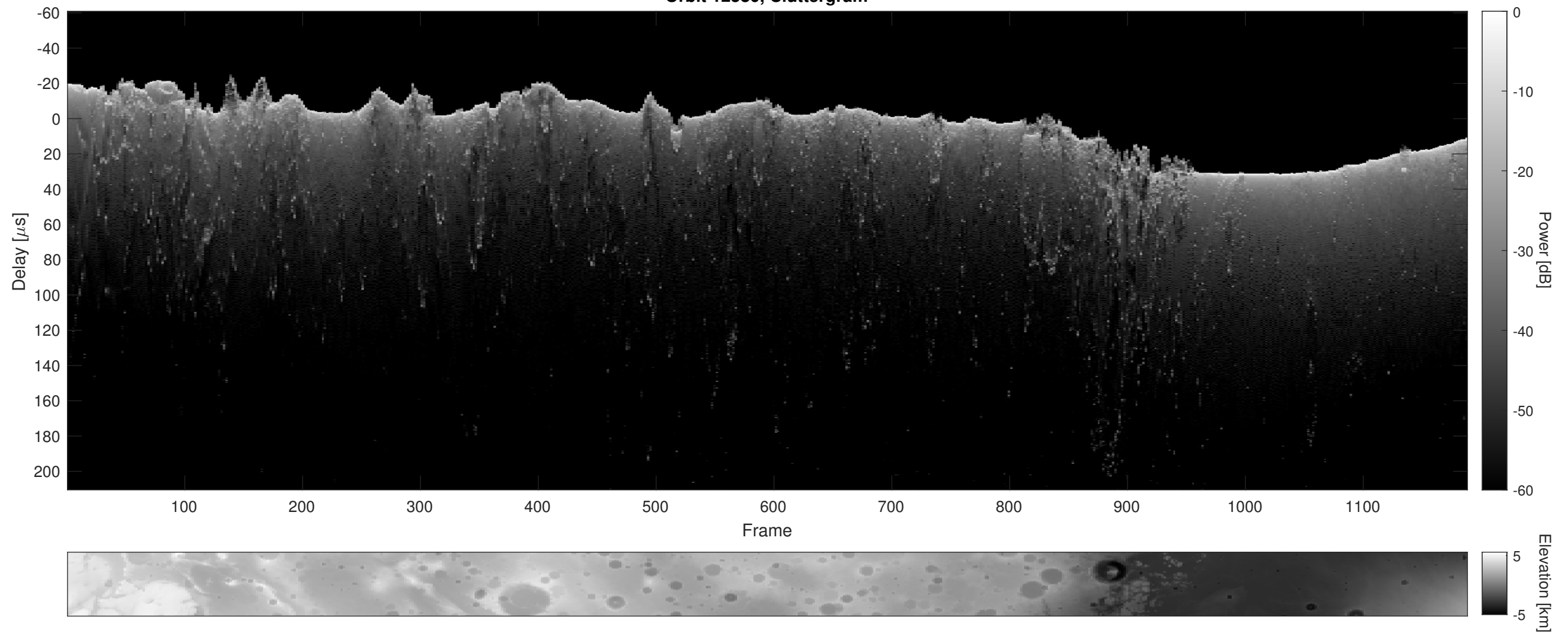
Orbit 12580, Cluttergram
