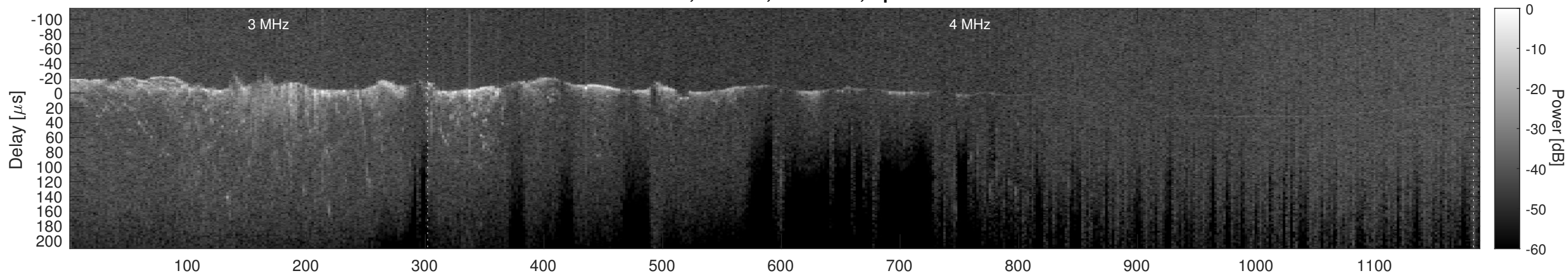
Orbit 12580, Cluttergram
