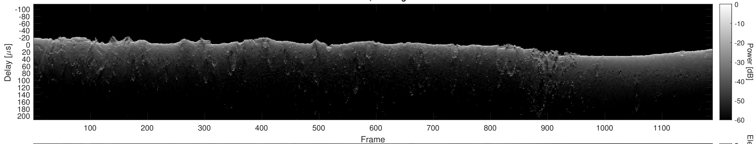
Orbit 12580, Cluttergram
