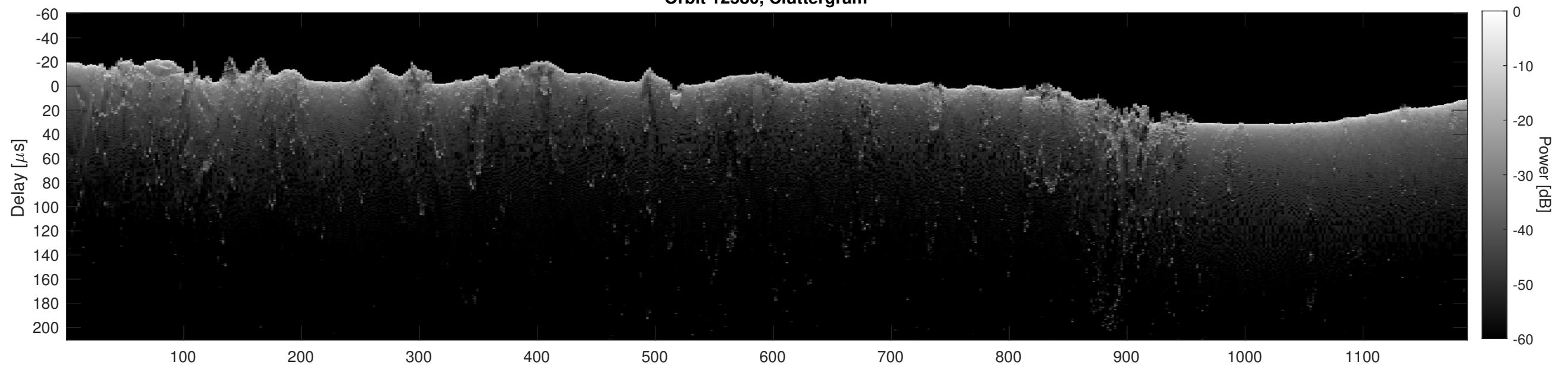
Orbit 12580, Cluttergram
