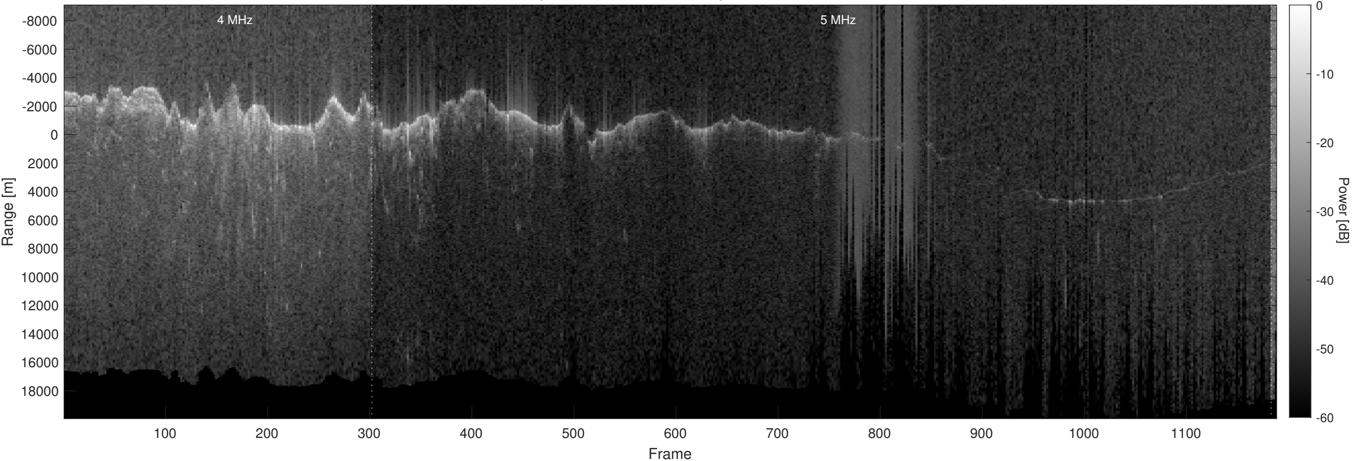
Orbit 12580, Optimized, No Window, Depth-Corrected, Channel 2
