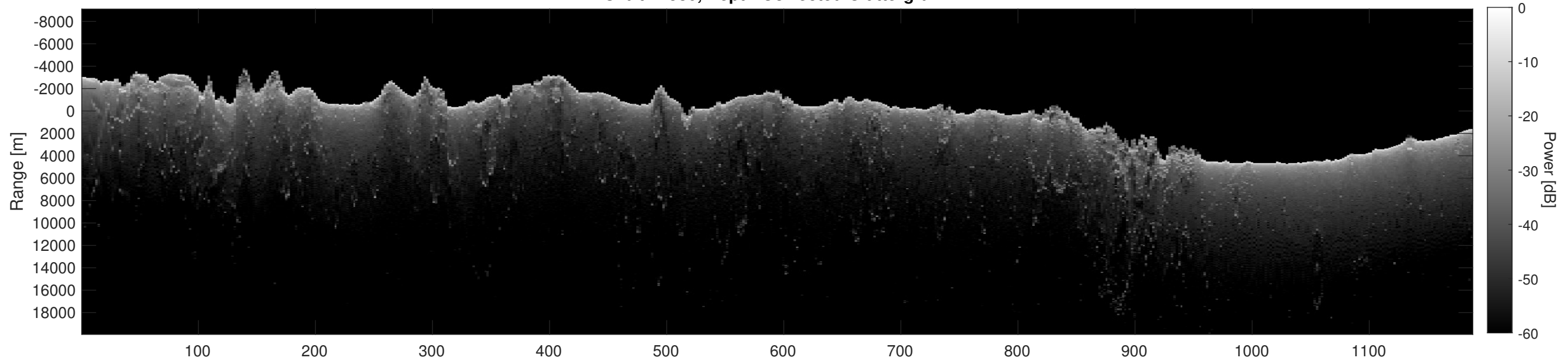
Orbit 12580, Depth-Corrected Cluttergram
