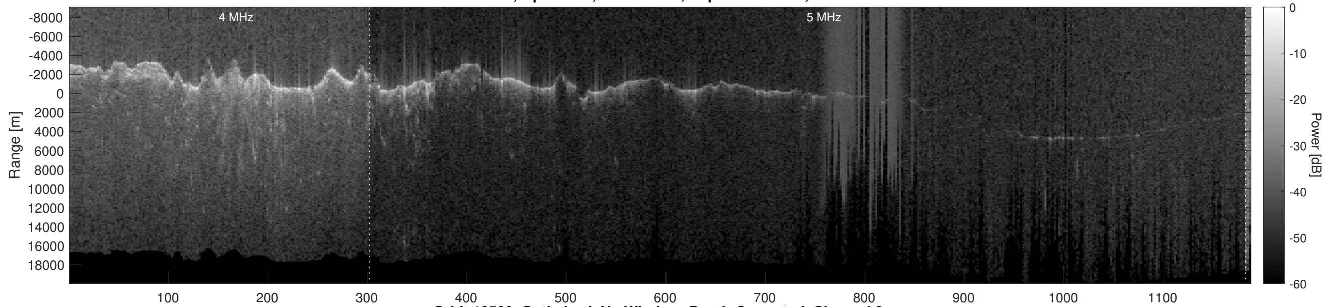
Orbit 12580, Optimized, No Window, Depth-Corrected, Channel 2
