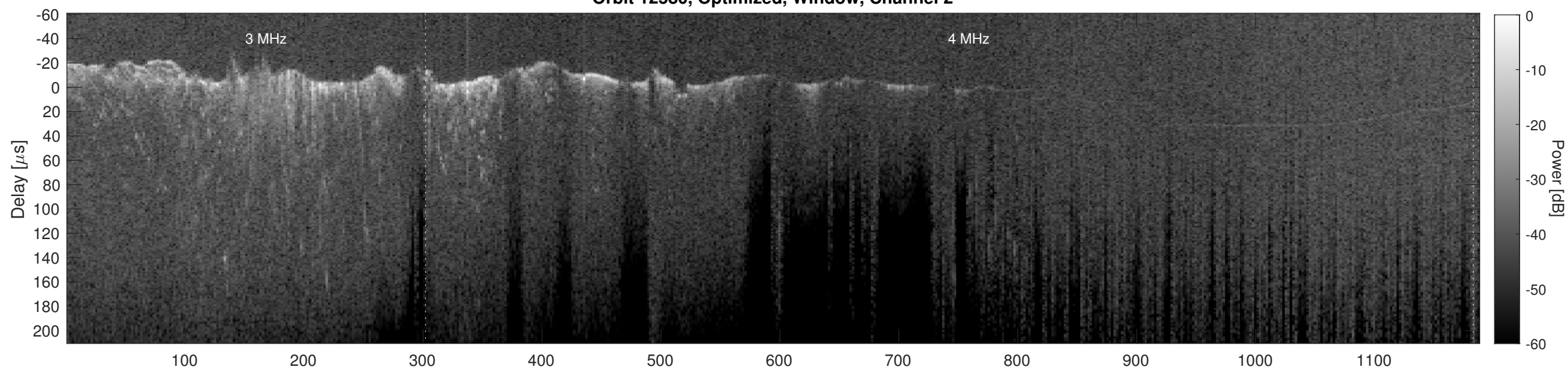
Orbit 12580, Cluttergram
