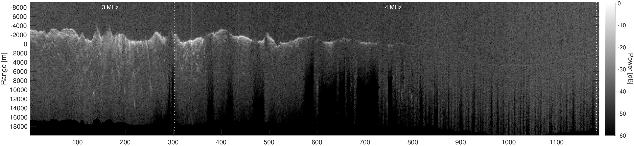
Orbit 12580, Depth-Corrected Cluttergram
