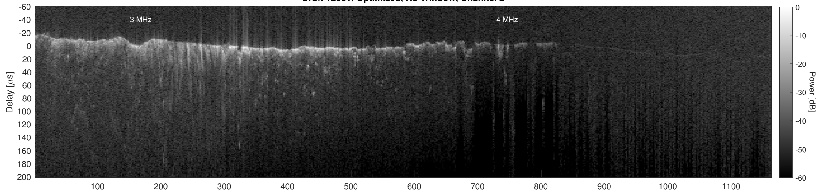
Orbit 12581, Cluttergram
