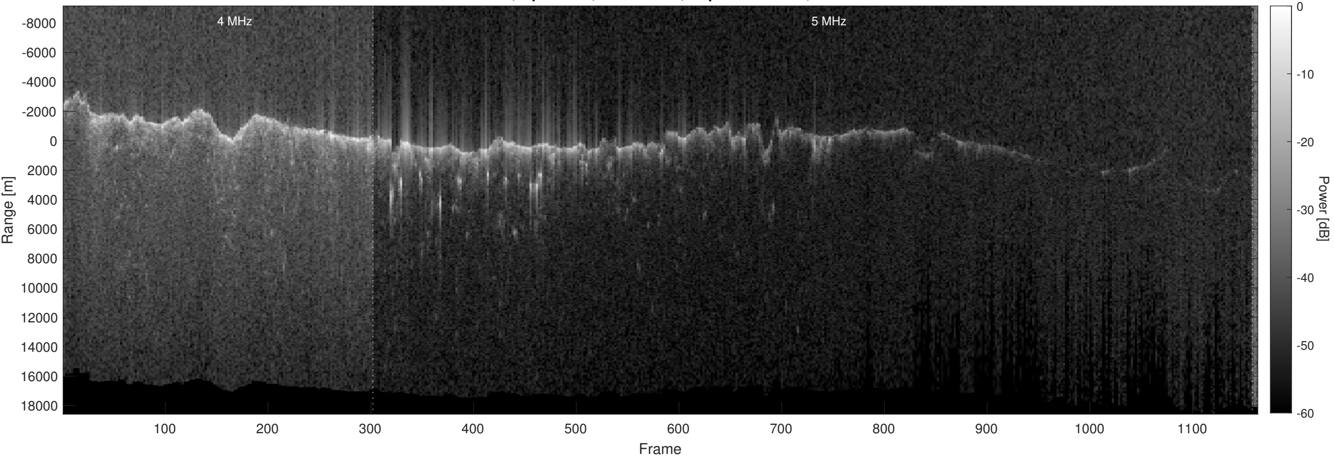
Orbit 12581, Optimized, No Window, Depth-Corrected, Channel 2
