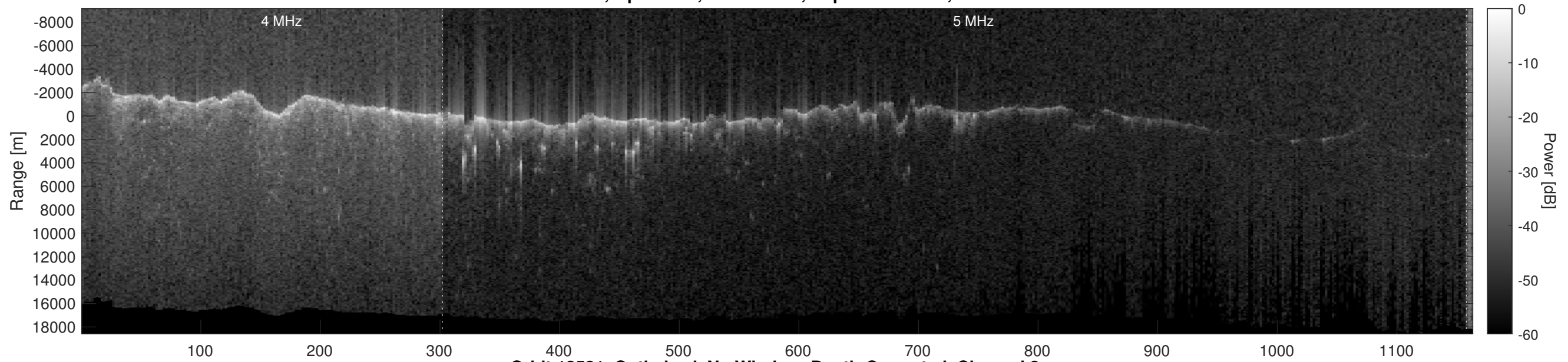
Orbit 12581, Optimized, No Window, Depth-Corrected, Channel 2
