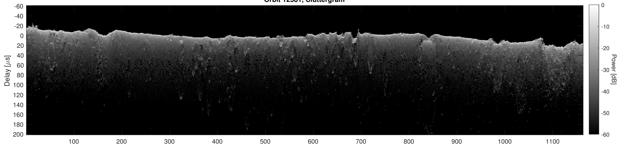
Orbit 12581, Cluttergram
