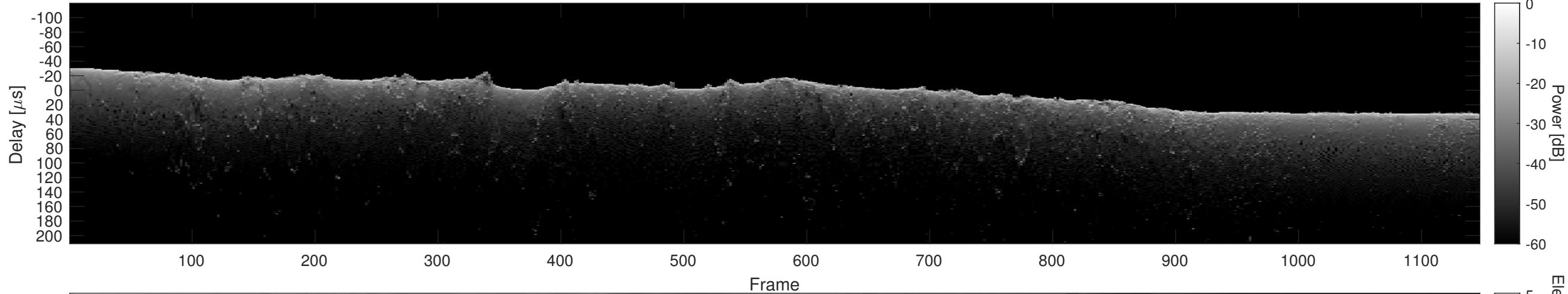
Orbit 12583, Cluttergram
