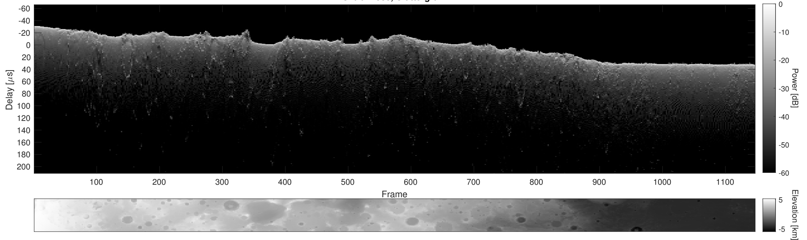
Orbit 12583, Cluttergram
