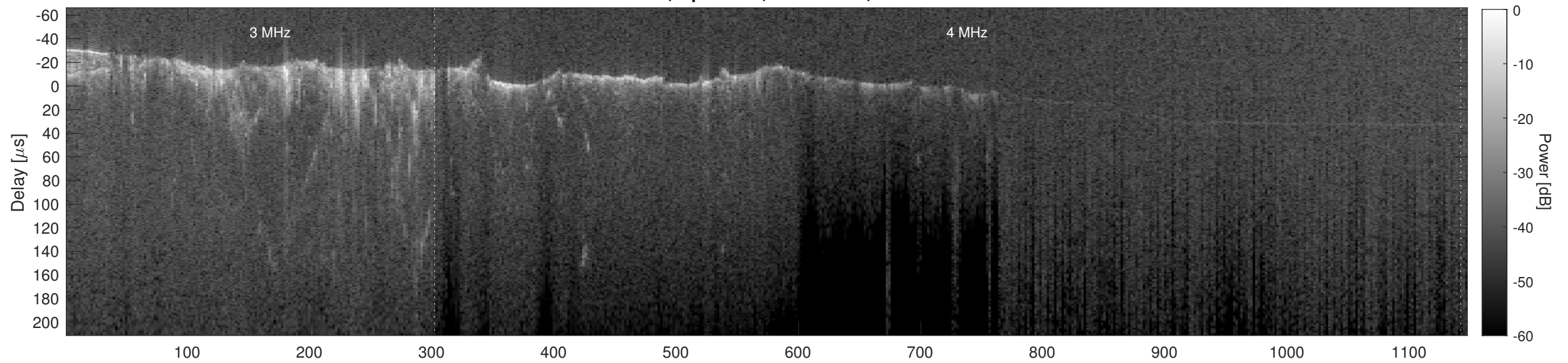
Orbit 12583, Cluttergram
