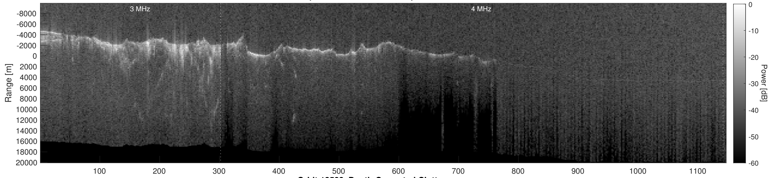
Orbit 12583, Depth-Corrected Cluttergram
