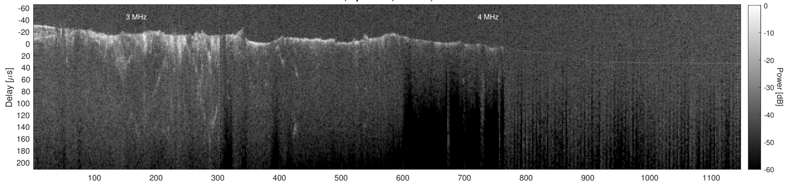
Orbit 12583, Cluttergram
