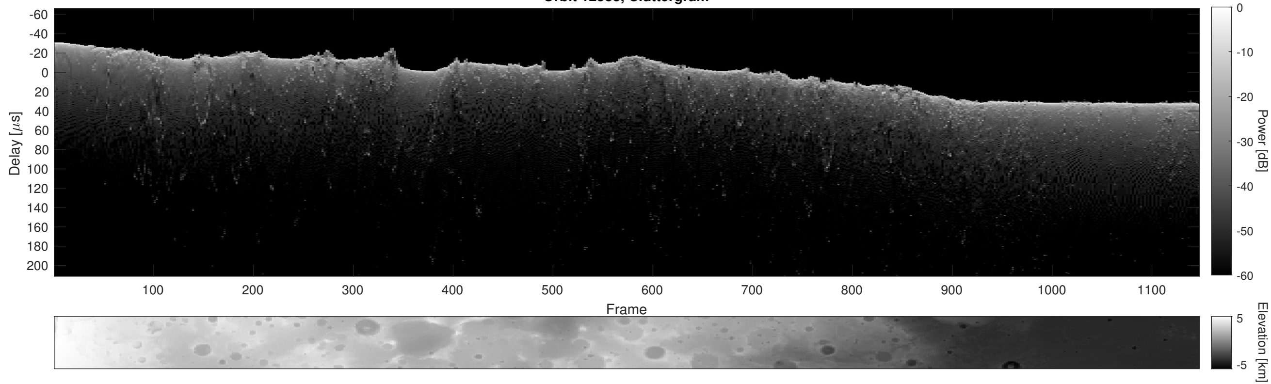
Orbit 12583, Cluttergram
