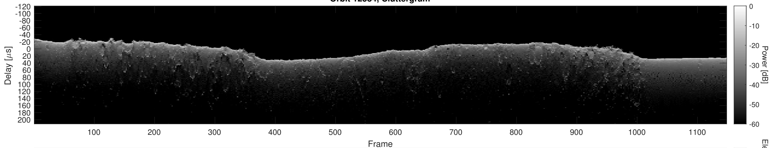
Orbit 12584, Cluttergram
