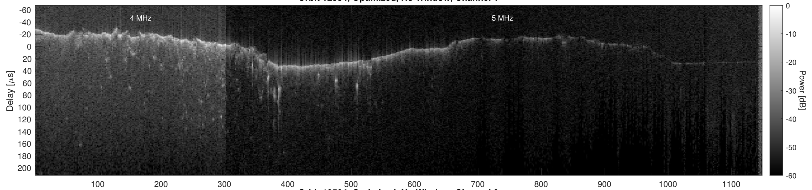
Orbit 12584, Optimized, No Window, Channel 2
