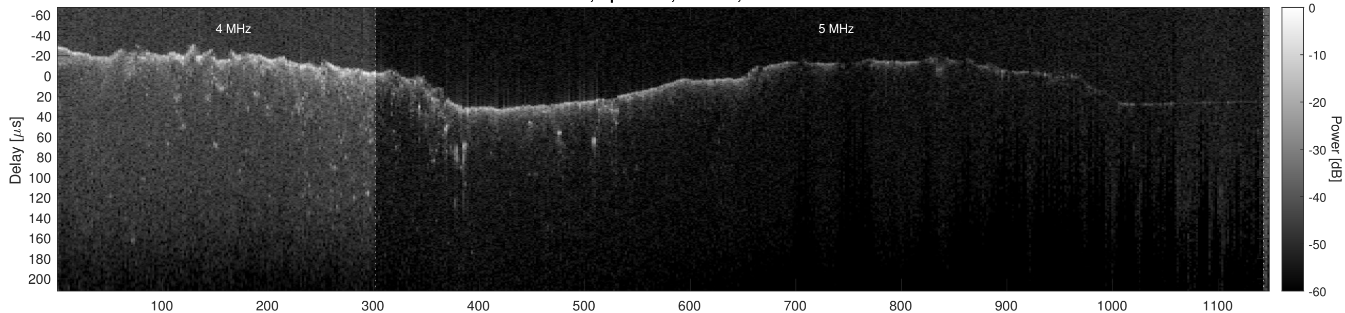
Orbit 12584, Optimized, Window, Channel 2
