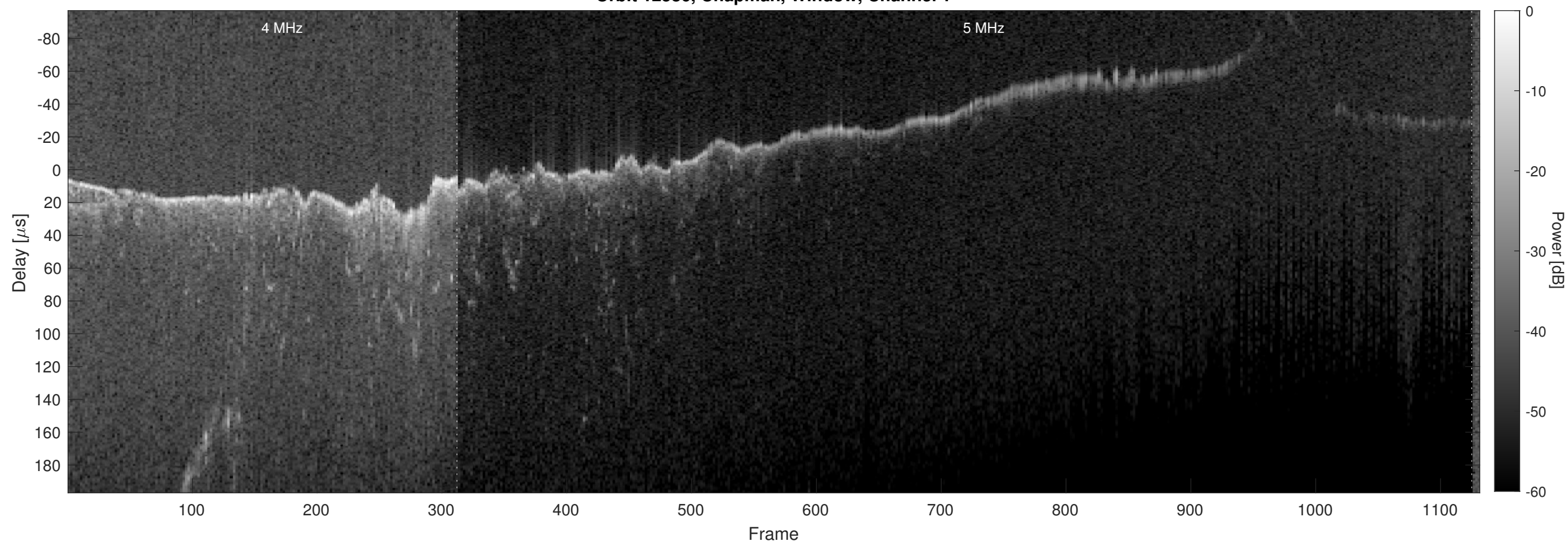
Orbit 12586, Chapman, Window, Channel 2
