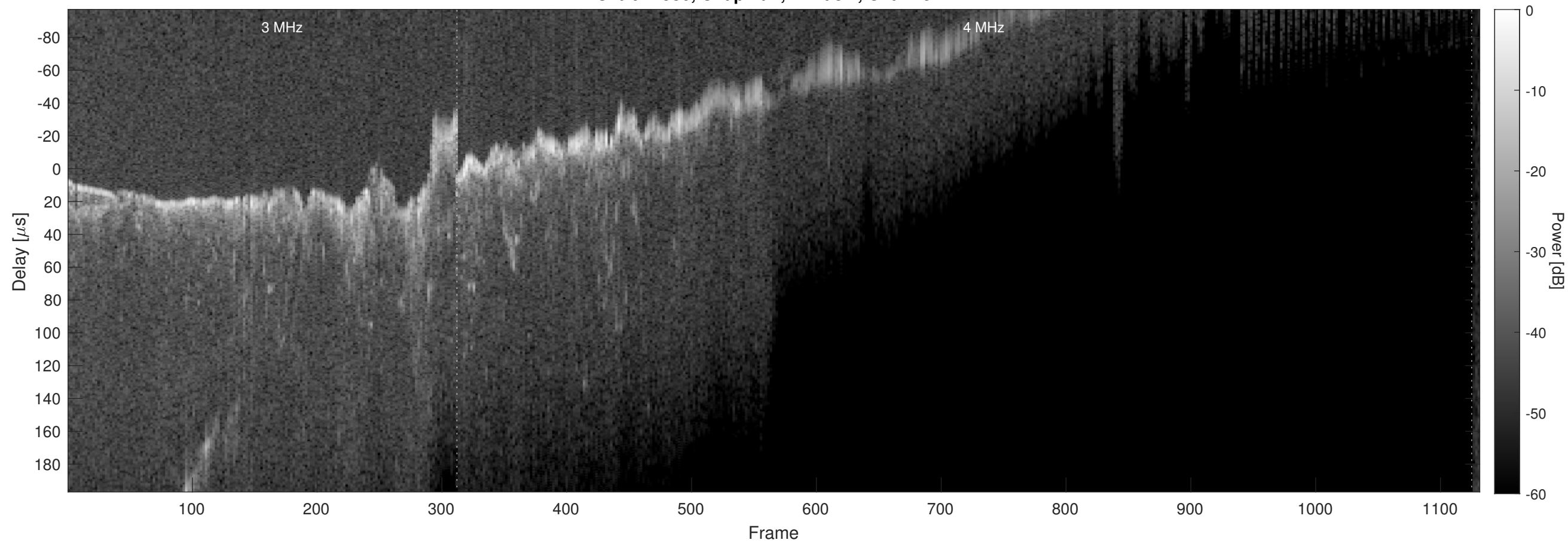
Orbit 12586, Chapman, Window, Channel 2
