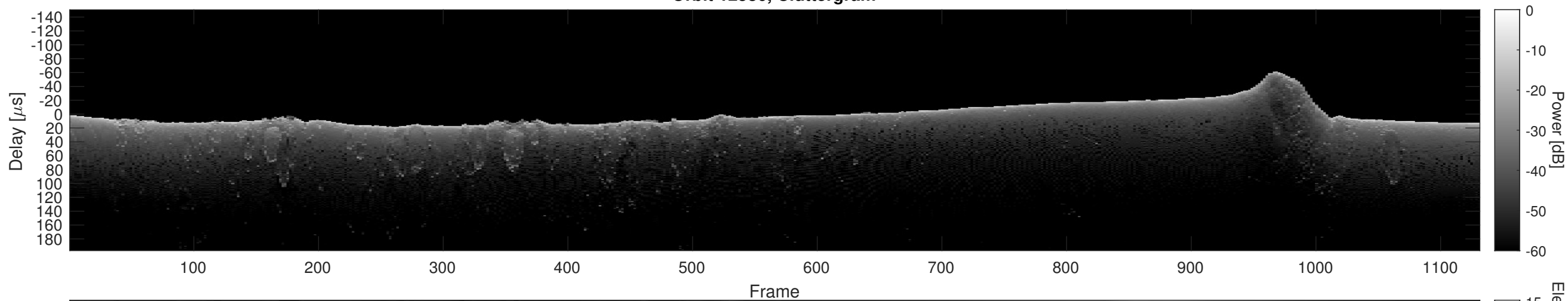
Orbit 12586, Cluttergram
