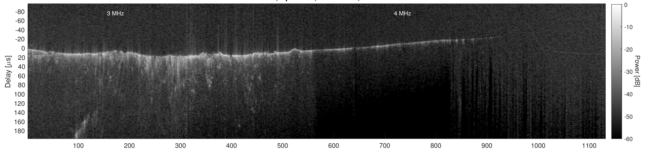
Orbit 12586, Cluttergram
