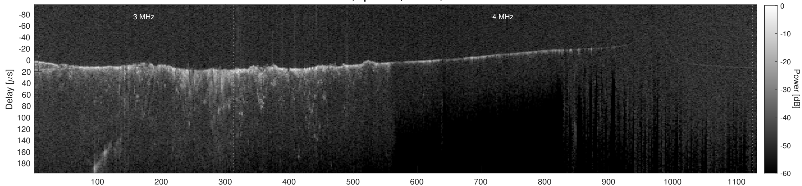
Orbit 12586, Cluttergram
