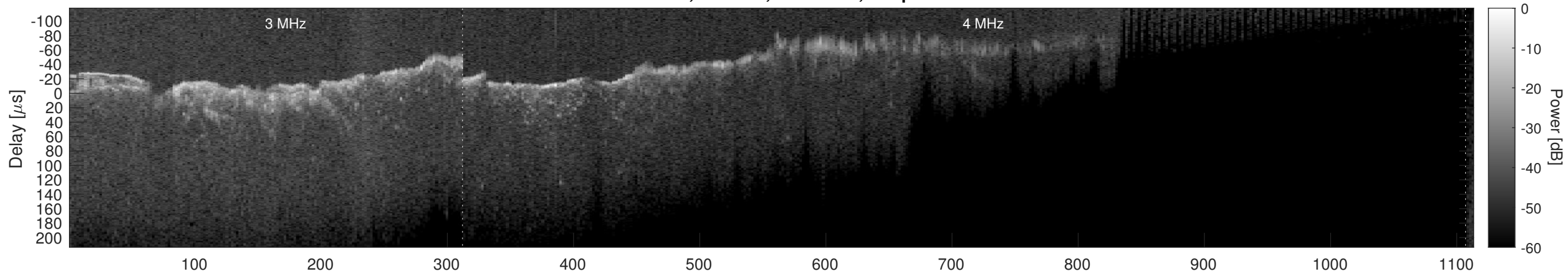
Orbit 12590, Window, Channel 2, Optimized
