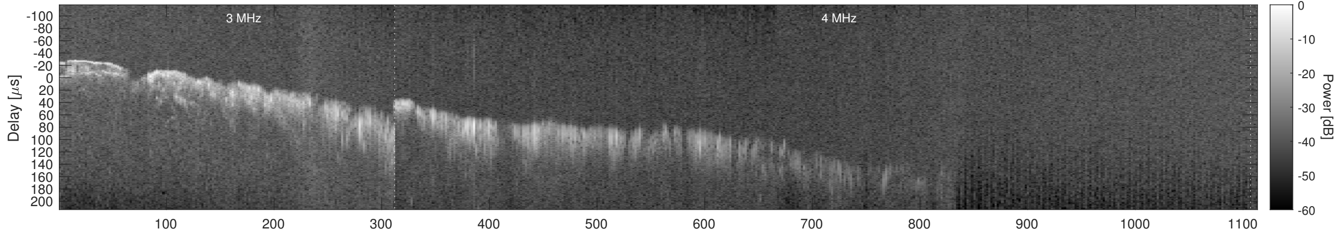
Orbit 12590, Window, Channel 2, Chapman
